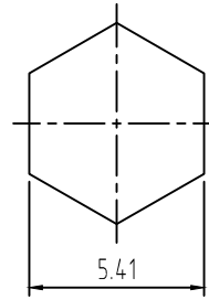
RECOMMENDED USE CRIMP TOOL DIE 0.213"
