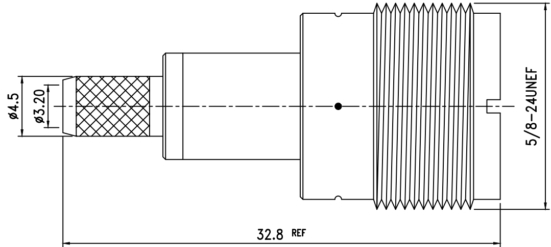
RECOMMENDED USE CRIMP TOOL DIE 0.213"
